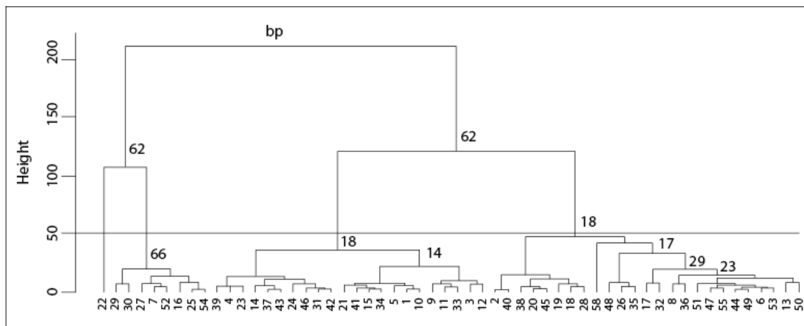
Figure 6. Classification dendrogram of 56 individuals belonging to eight papaya genotypes based on the variables studied using Ward's minimum variance algorithm and the Euclidean metric distance. The bp values in the branches of the larger groups indicate the result of the Bootstrapping.
