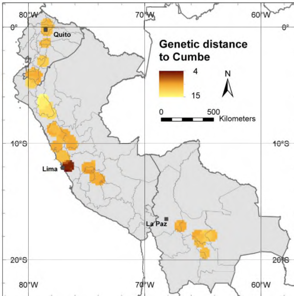
Figure 7. Genetic distance to the Peruvian cultivar 'Cumbe'. This maps shows the average genetic distance (GD) to the cultivar 'Cumbe', in each 10-minutes cell with 20 or more trees applying a one-degree circular neighborhood. As reference of the cultivar, the 'Cumbe' accession from the collection la Mayora, Malaga, Spain, was used. doi:10.1371/journal.pone.0029845.g007
